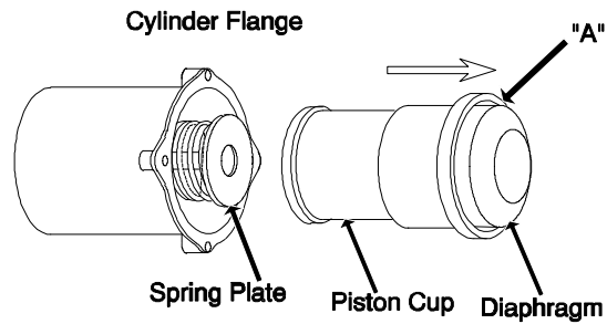
Figure 2: Diaphragm Assembly
