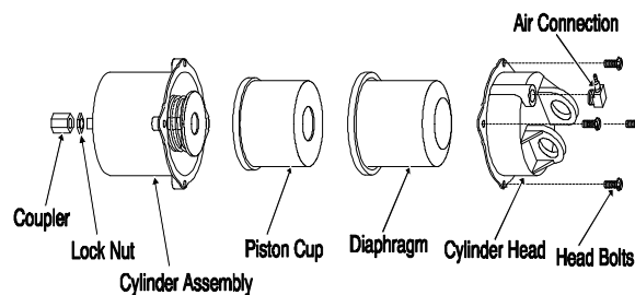
Figure 1: Actuator Components
